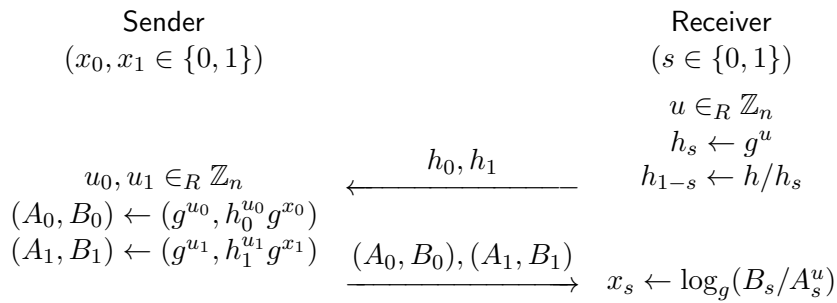
FIGURE 7.2: \binom{2}{1} -OT protocol
